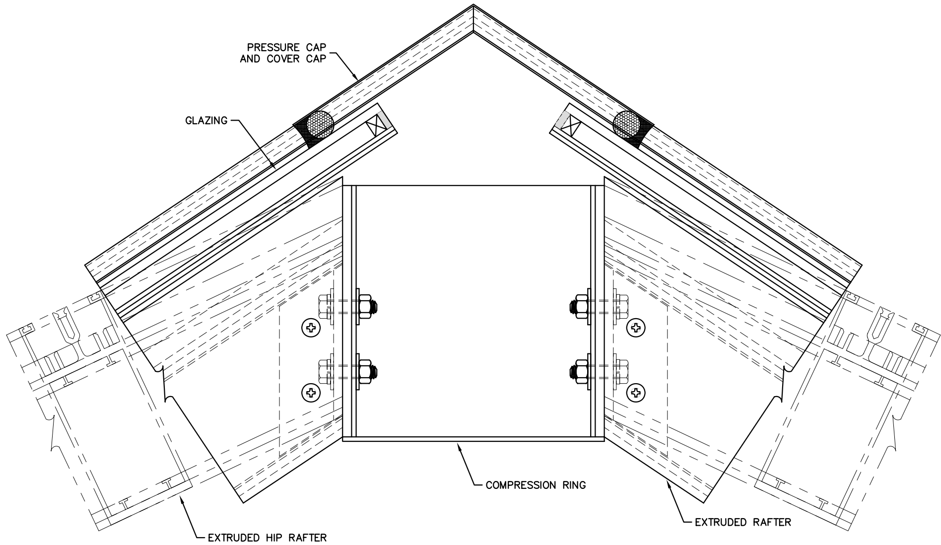
RIDGE DETAIL
