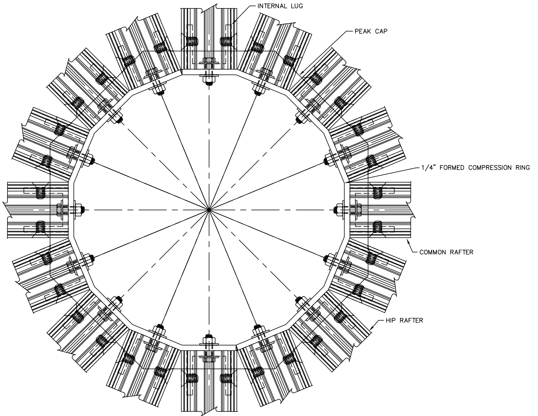
COMP. RING DETAIL
