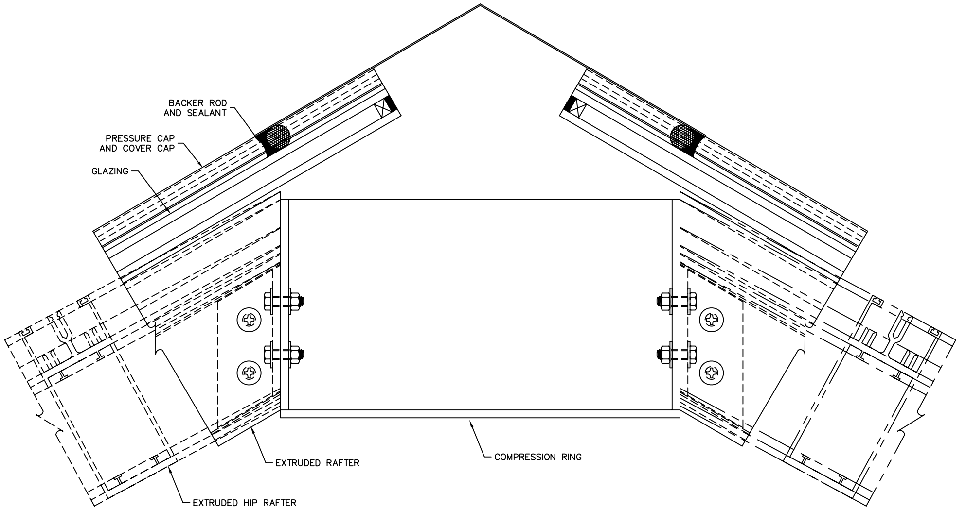
○ ——— COMP. RING ———— DETAIL
