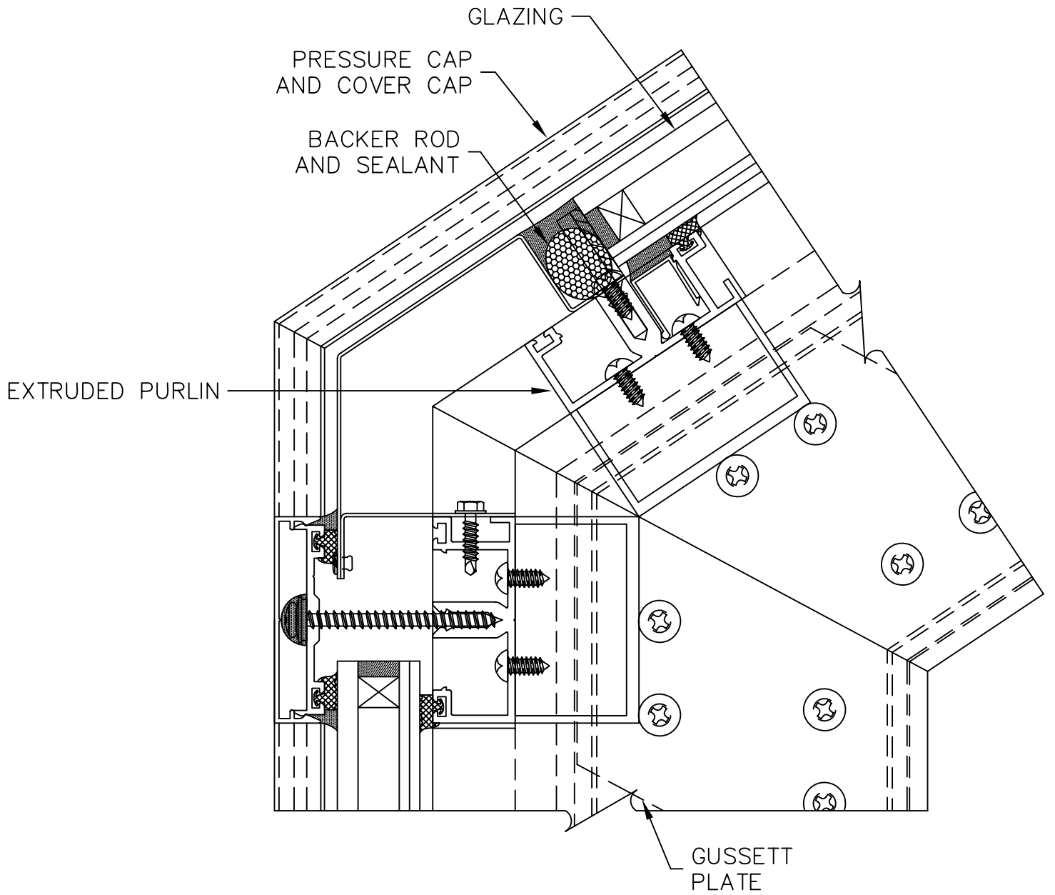
KNEE DETAIL
