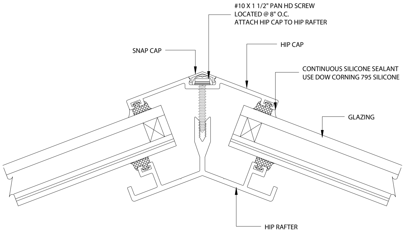
HIP RAFTER DETAIL
